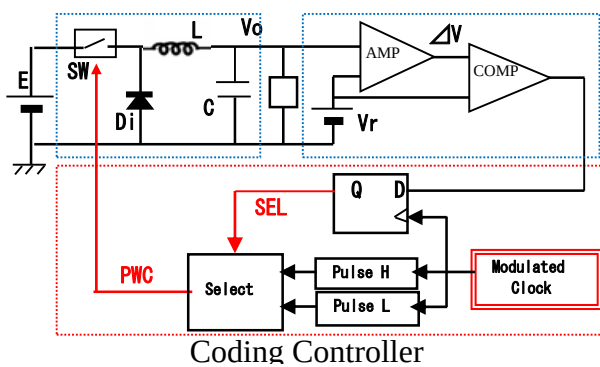
Fig.5 Converter with PWC control
