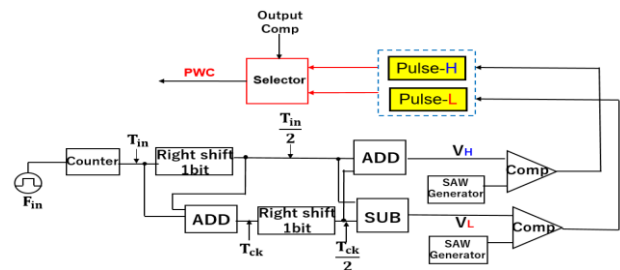
Fig.6 Automatic PWC method of the direct method
