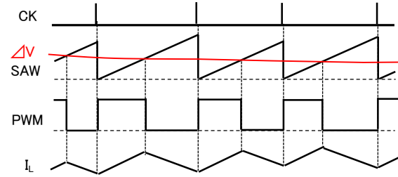
Fig.1 Switching buck converter with PWM signal Fig.2 Waveform of switching buck converter
